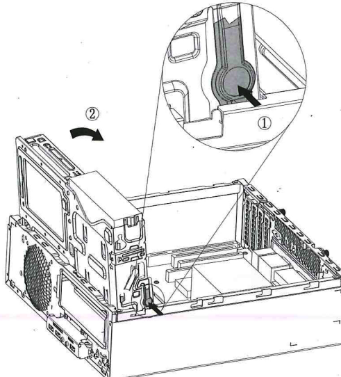
Press ODD lock ① Close ODD bracket
