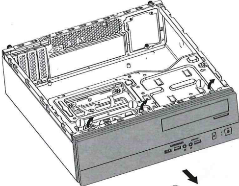
How to disassemble front panel
