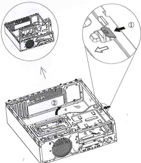
Press the Retaining Clip ① Pivot the drive bay upward
