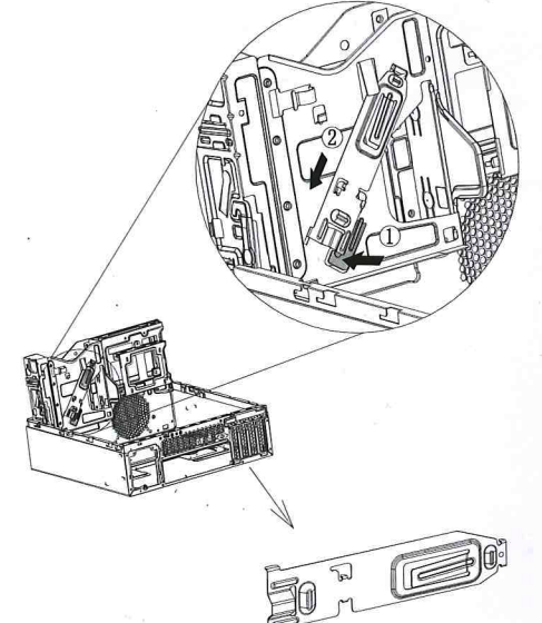
Disassemble ODD Retainer
