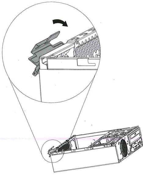
How to install PCI Cards
