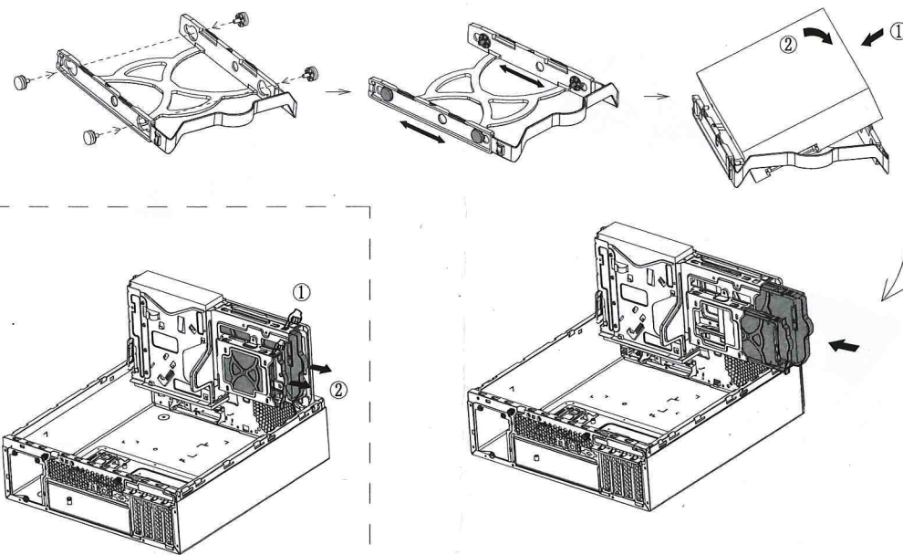
Install 3.5"HDD/2.5"HDD/SSD
