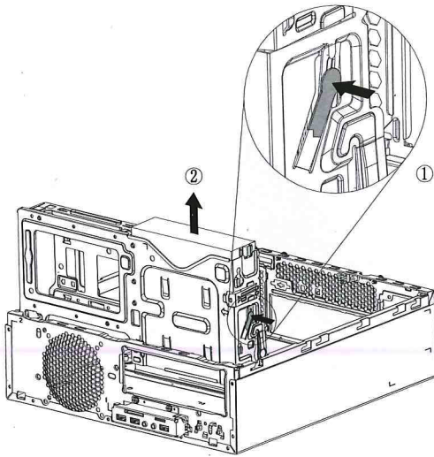
Disassemble CD-Rom
