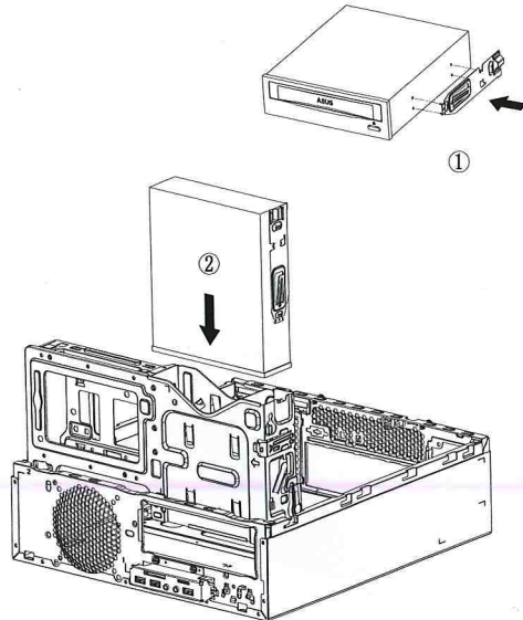
Install CD-Rom
