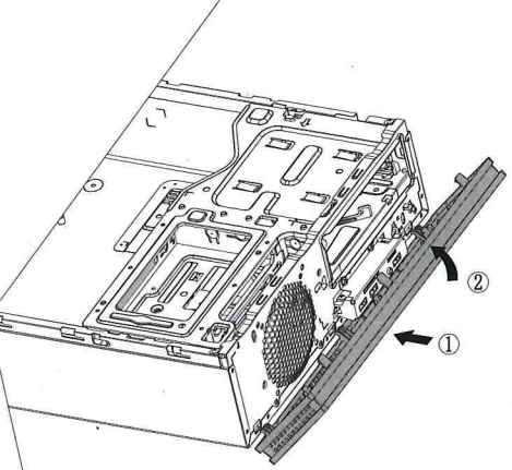
How to install front panel
