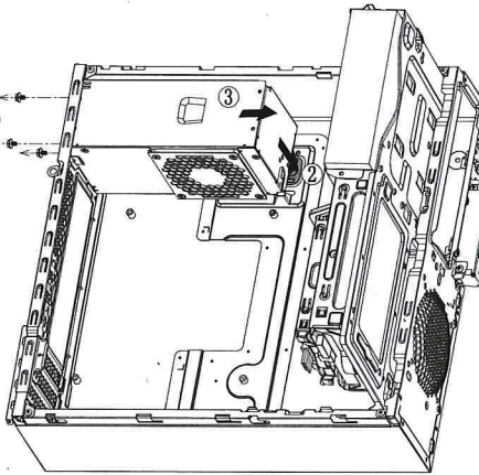
Disassemble power supply
